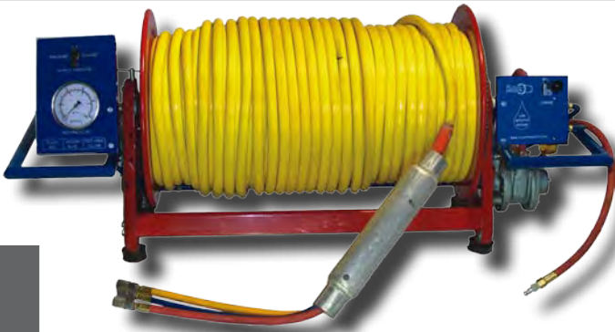
Leak Location Reel PART # 1100-300
